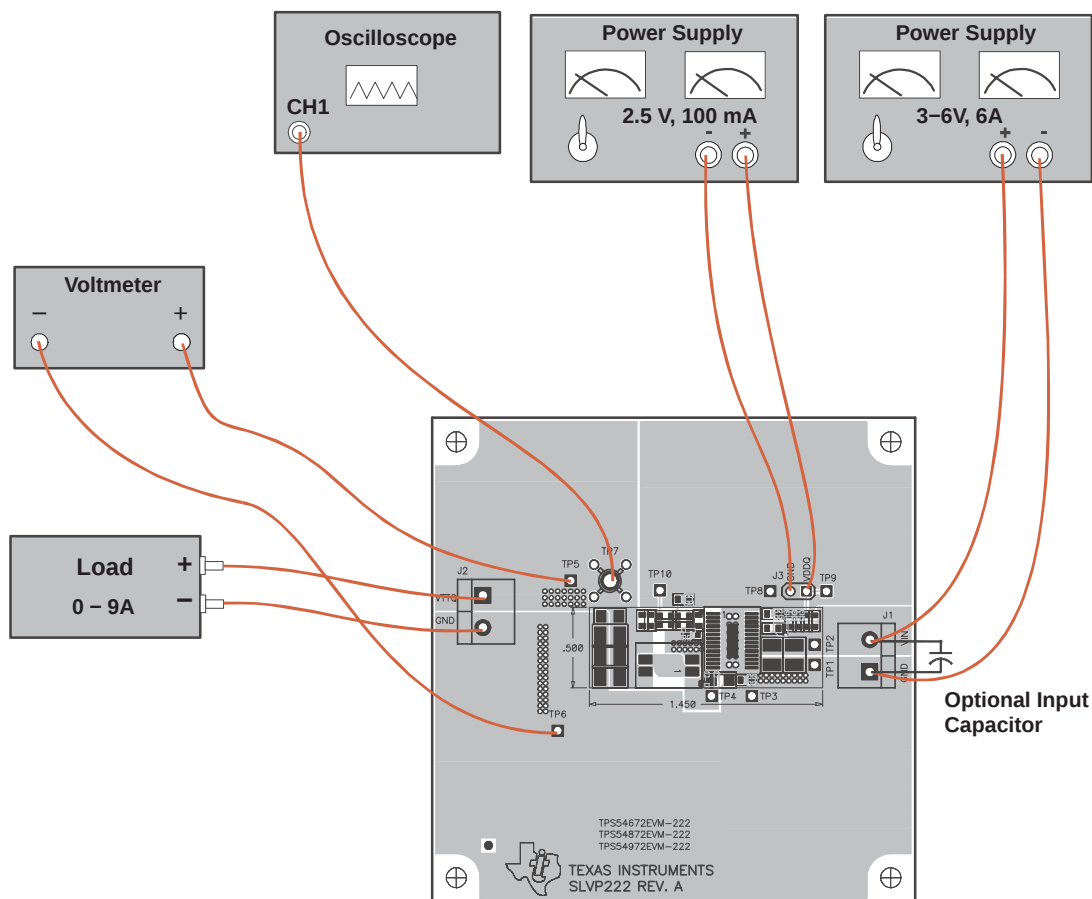
Figure 2-1. Connection Diagram
